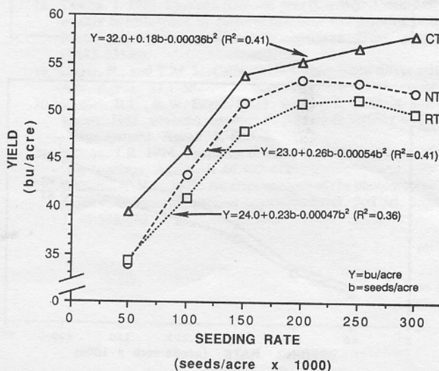
Fig. 3. Study 2, soybean yield and prediction models in response to seeding rate for no-tillage (NT), reduced tillage (RT), and complete tillage (CT) systems, averaged for two varieties over 3 yr at Arlington, WI.
